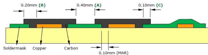
PCB cross-section
